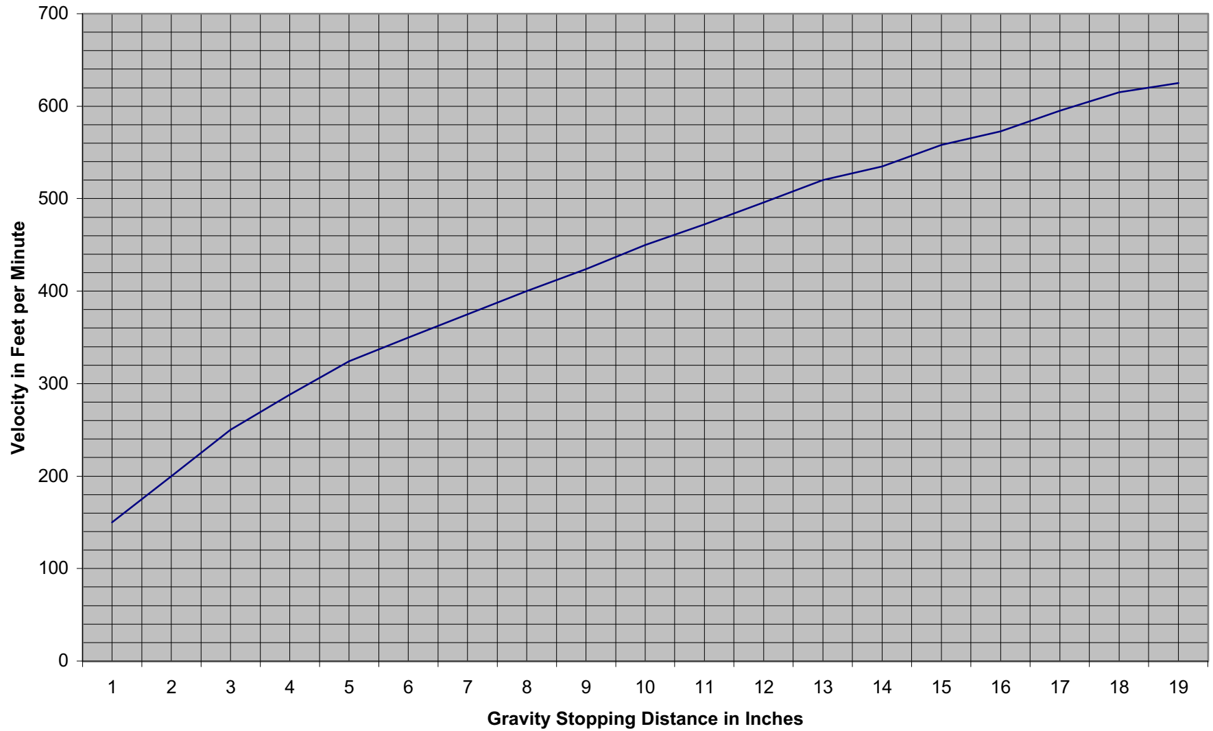
Fig. 2 Gravity Stopping Distance
