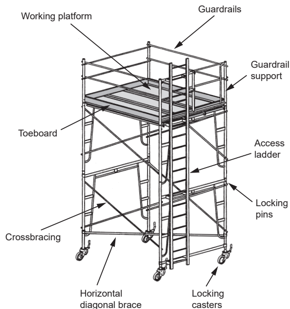
Illustration 9 | Tower and Rolling Scaffold
